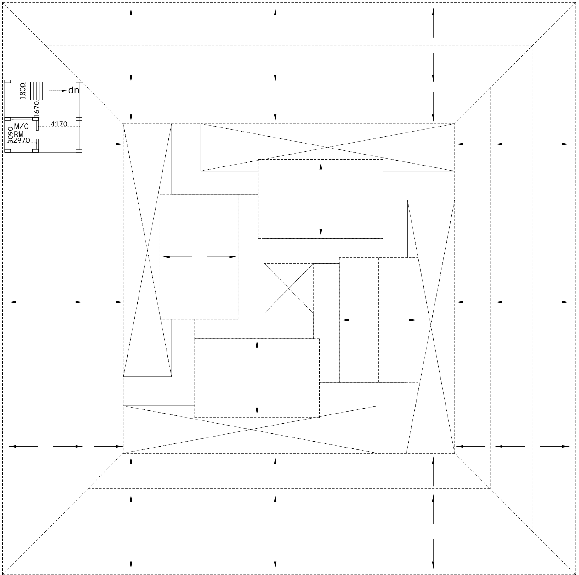
ROOF PLAN
